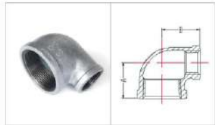
Fig.90R 90° Elbow, Reducing
