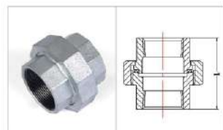
Fig.340 Union,conical seat
