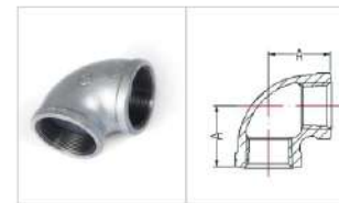
Fig.90 90° Elbow, Equal
