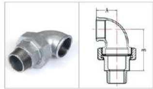
Fig.98 M&F Conical Union Elbow
