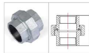
Fig.331 Union,flat seat,M&F
