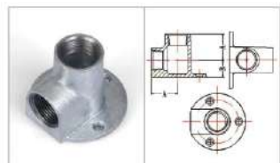
Fig.1221 Banded Side Outlet Elbow
